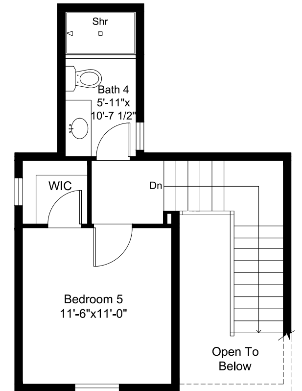
ATTIC FLOOR
