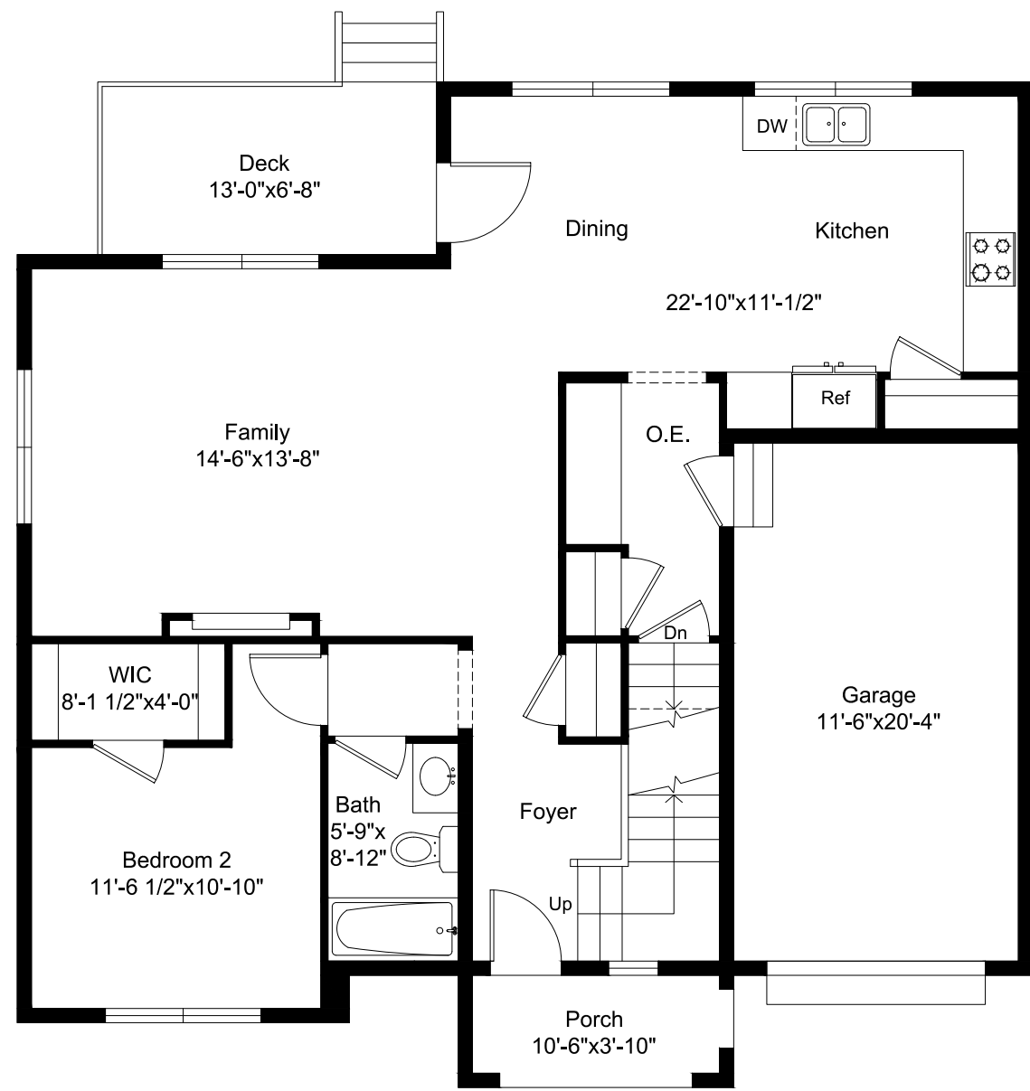
MAIN FLOOR
