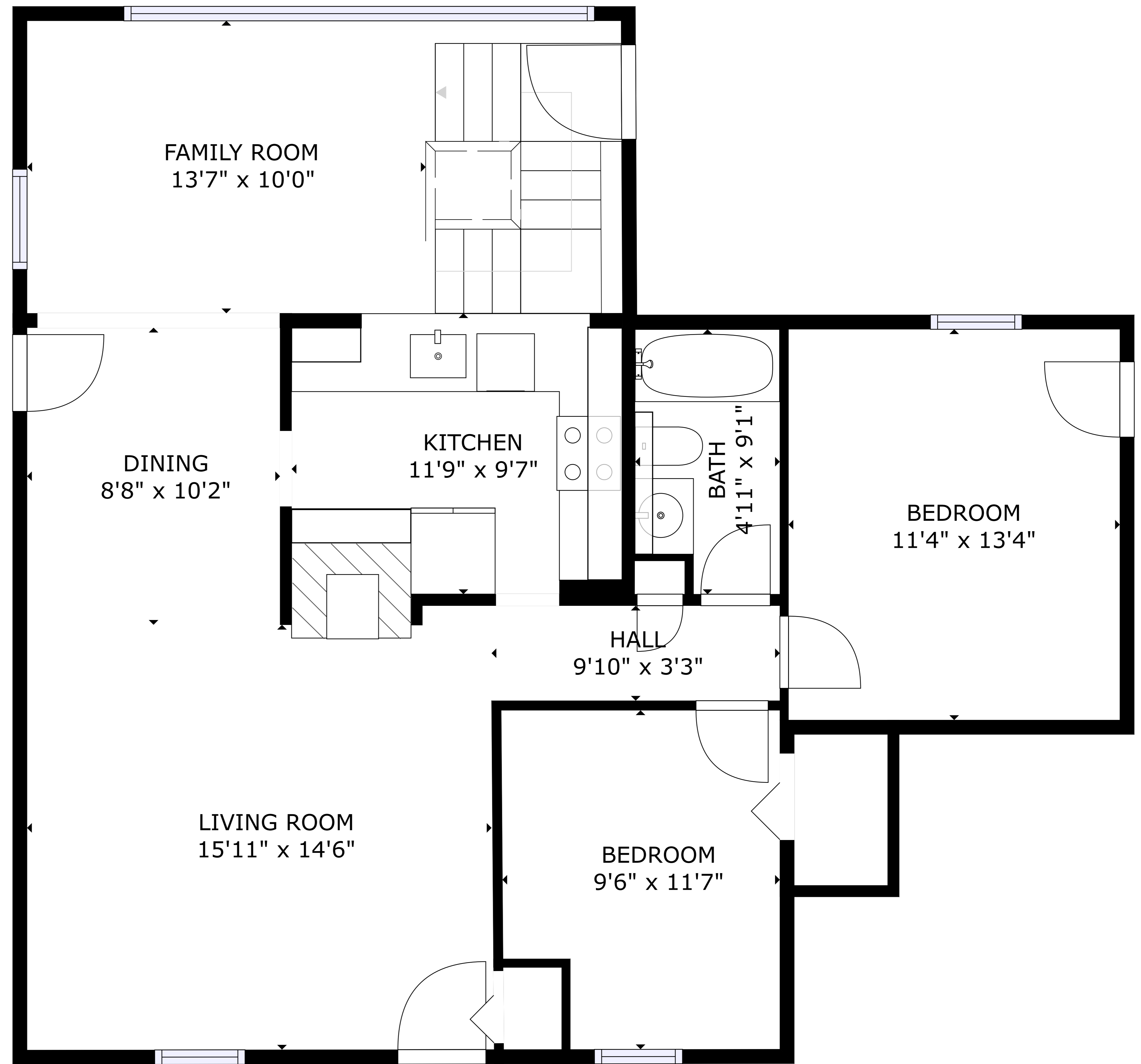
FIRST FLOOR
