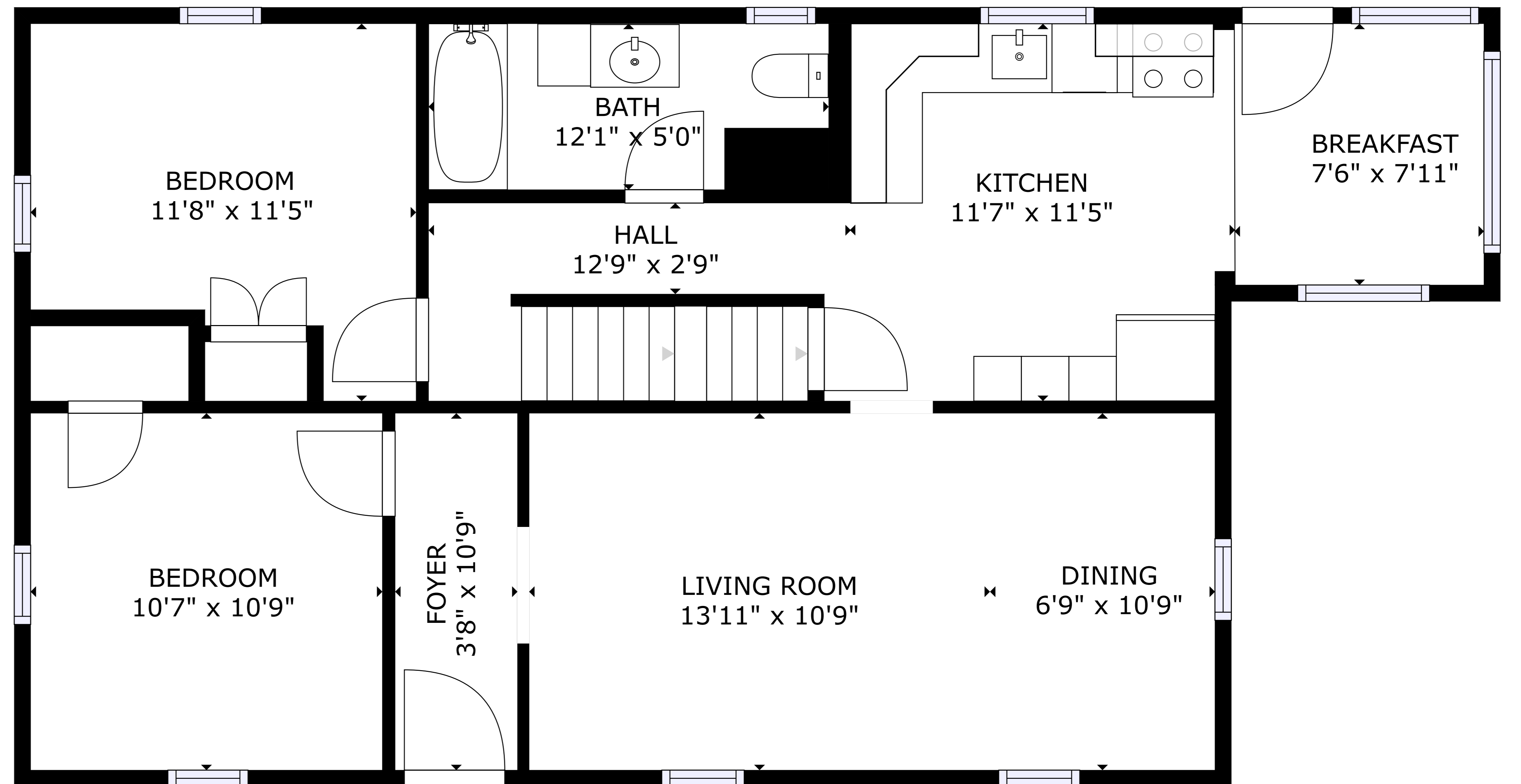
FIRST FLOOR
