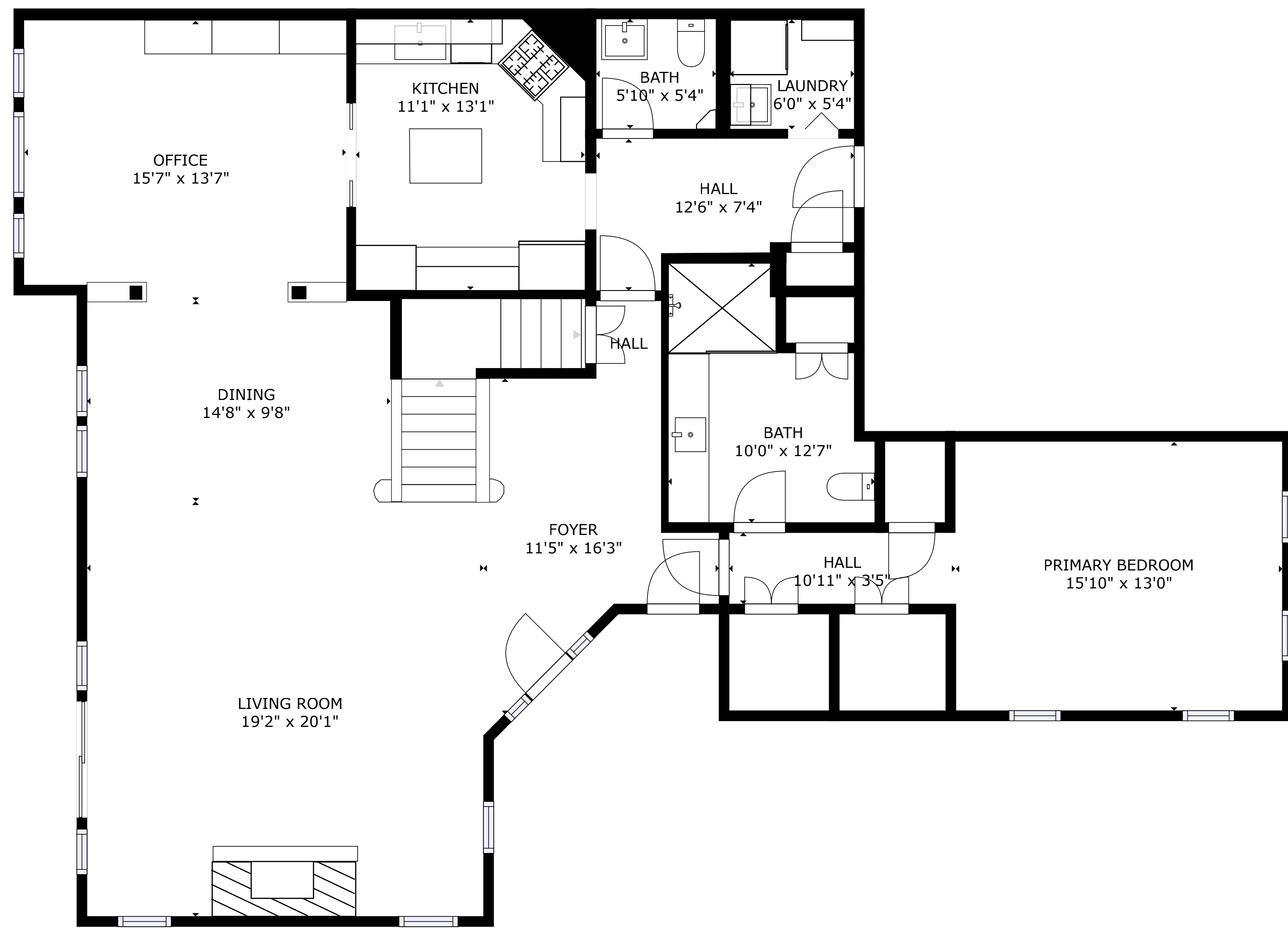
FLOOR 2
