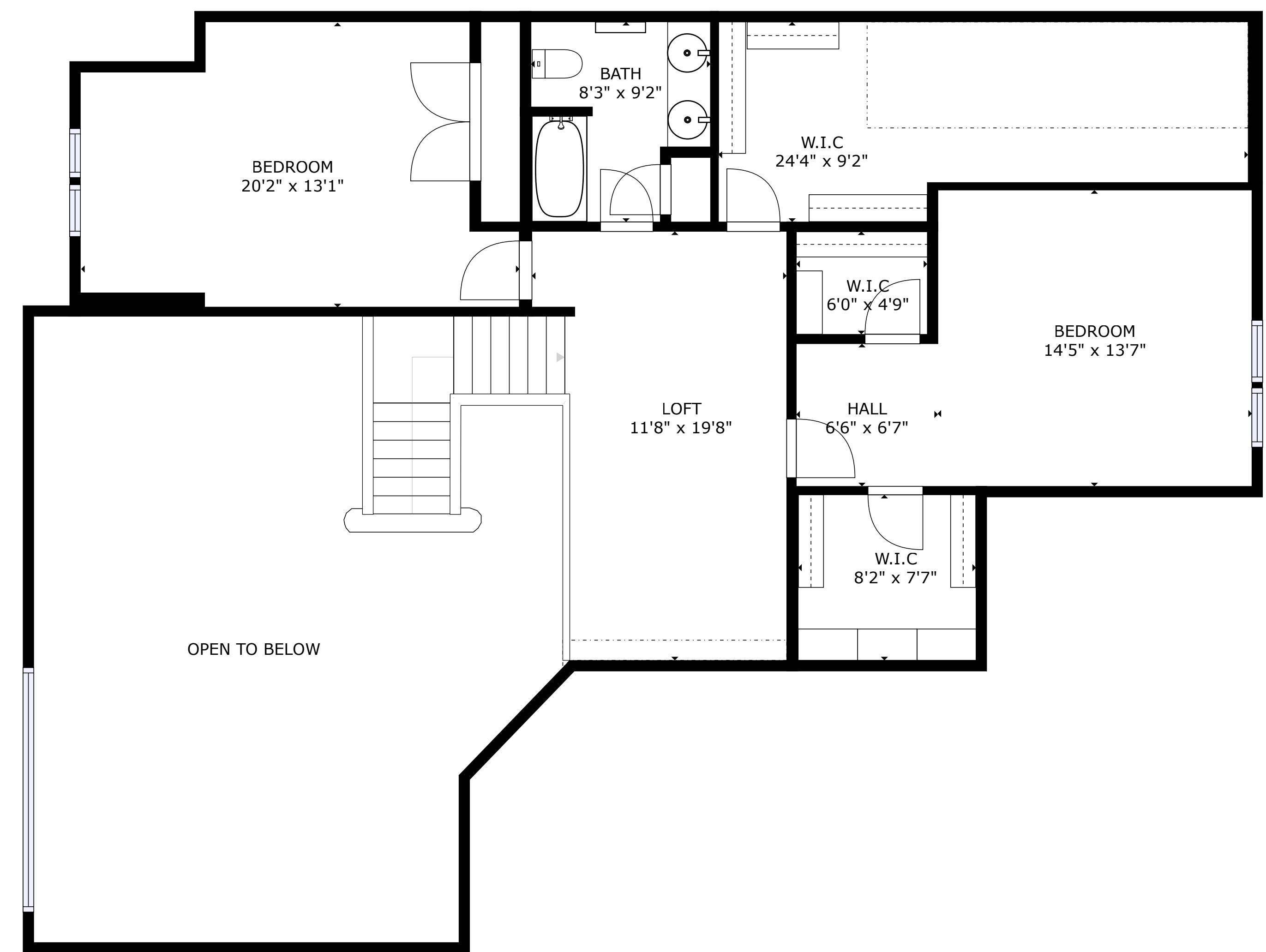
FLOOR 3
